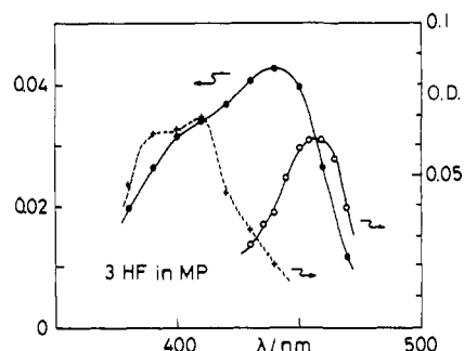
Figure 2. Time-resolved transient absorption spectra of the MP solution of 3-hydroxyflavone at room temperature: (●) depicted at 300-ns delay after a laser excitation; (○) at ~13-ns delay; (+) at ~50-ns delay.
